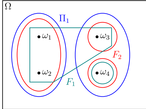
Figure 10: The notion of “individually more informative than” does not imply “finer than”, though the latter does imply the former. In this figure, F_2 (red) strictly refines F_1 (green) and \Pi_1 (blue), but for every deterministic \tau_2 , there exists a deterministic \tau_1 such that \Pi_1 \vee \tau_1 = \Pi_1 \vee \tau_2 , so F_1 is individually more informative than F_2 .
