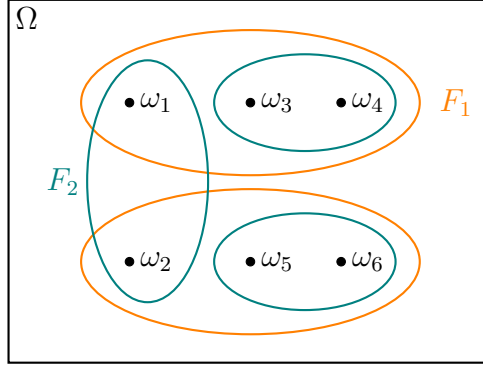
Figure 14: Refinement in every CKC does not imply IMI. Suppose \Pi_1 = \{\{\omega_1, \omega_2\}, \{\omega_4, \omega_5\}, \{\omega_3, \omega_6\}\} and \Pi_2 = \{\{\omega_1, \omega_2\}, \{\omega_3, \omega_4\}, \{\omega_5, \omega_6\}\} . There are two CKCs, \{\omega_1, \omega_2\} and \{\omega_3, \omega_4, \omega_5, \omega_6\} . Consider F_1 (orange) and F_2 (teal) depicted in the figure. Despite F_1 refines F_2 in every CKC, F_1 is not individually more informative than F_2 .
