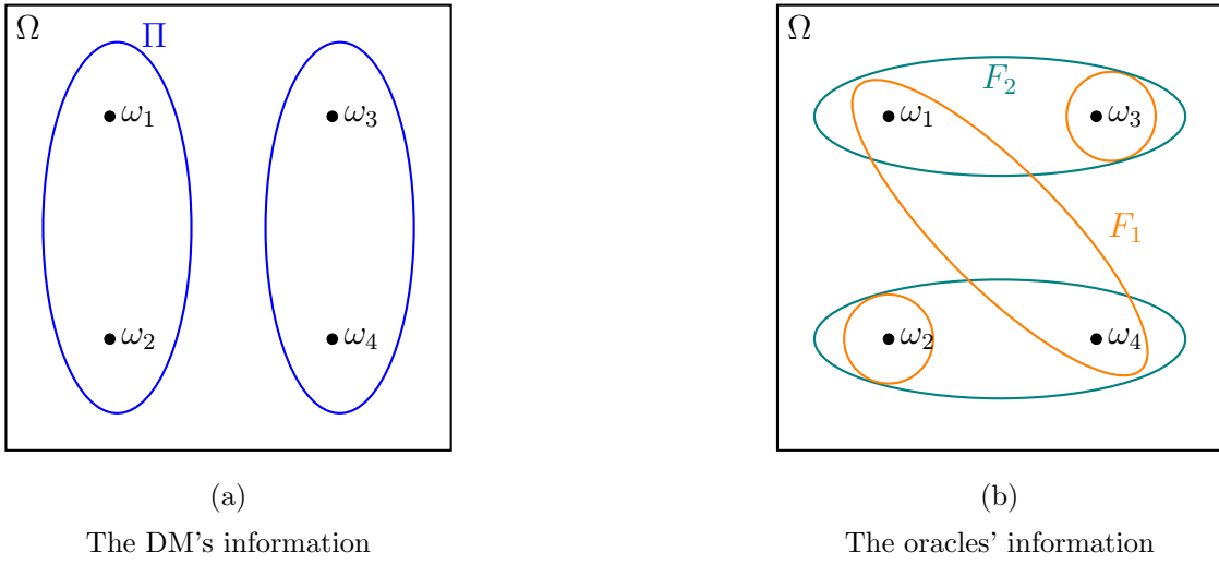
Figure 5: On the left, Figure (a) illustrates the information structure of the DM (blue). On the right, Figure (b) portrays the information structure of Oracle 1 (orange) and Oracle 2 (green).
