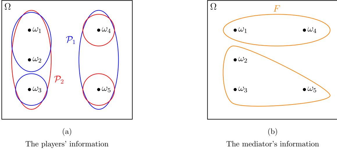
Figure 3: On the left, Figure (a) illustrates the information structure of player 1 (blue) and player 2 (red). On the right, Figure (b) portrays the information structure of the mediator (orange).
